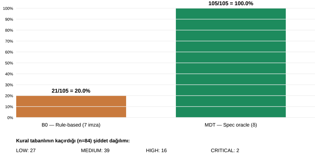
Şekil 7: Tespit completeness — kural-tabanlı (B0) vs. spec-oracle (MDT)
