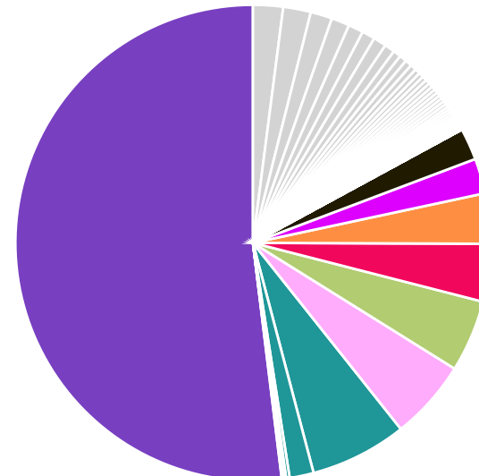
ME-ITS
