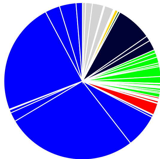
PB
