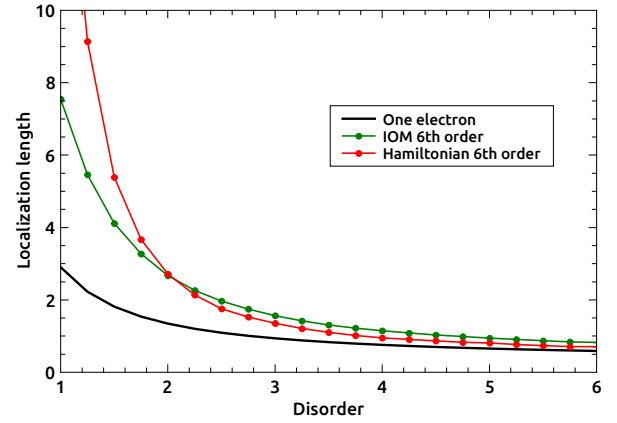
Figure 10 Localization length as a function of disorder for the IOMs and the Hamiltonian, when we include terms up to 6th order. For comparison, we included the one-electron localization length.
