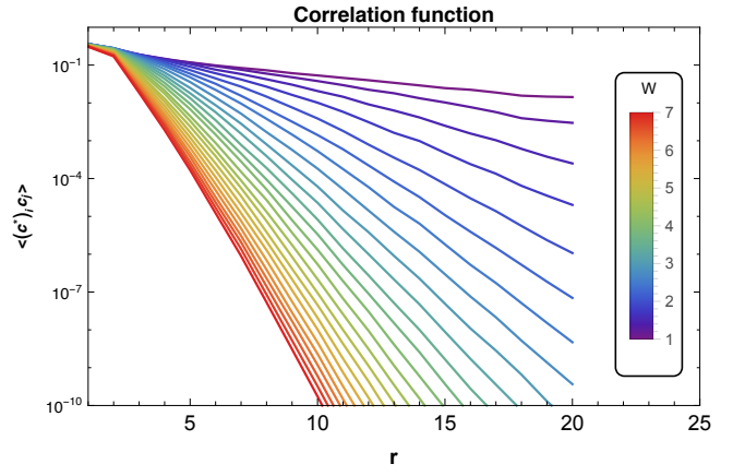
Figure 6 Spatial dependence of the correlation function Eqn. (41) for various disorder strengths W .
