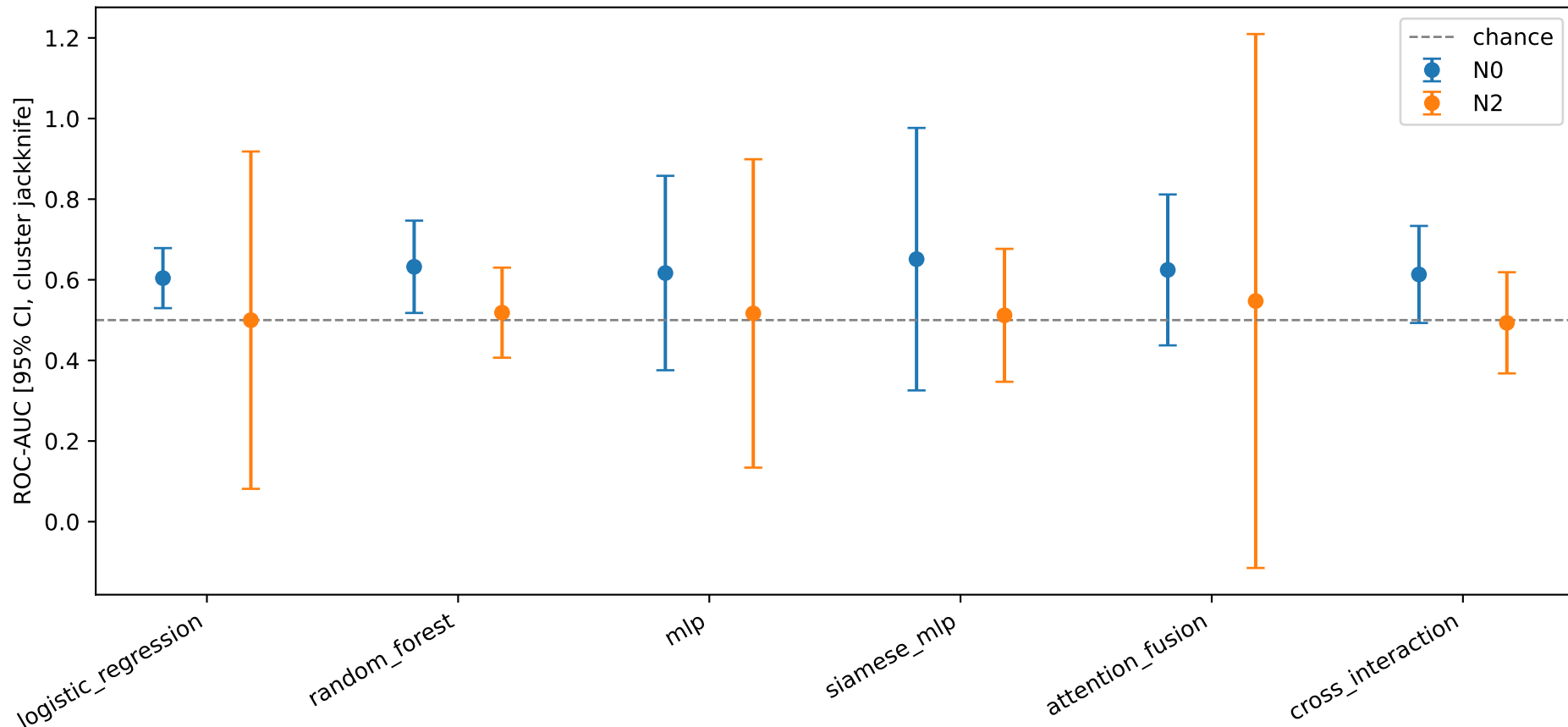
95% CIs, R3, connected-component cluster jackknife
