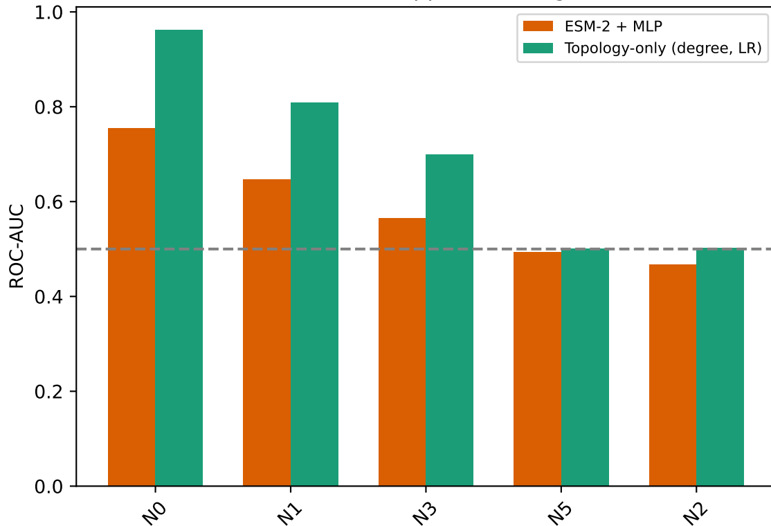
Exp A: trained on N0, evaluated on swapped test negatives
