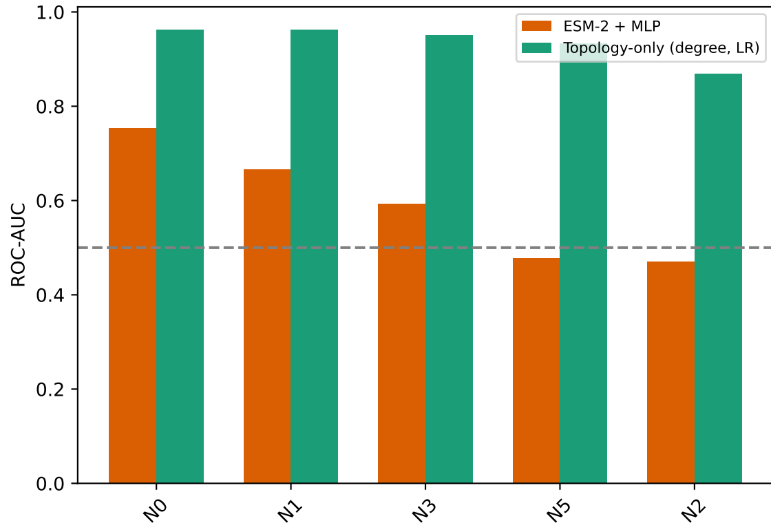
Exp B: trained on each negative set, evaluated on N0 (common benchmark)
