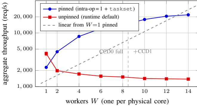
Fig. 2. Aggregate throughput versus fleet size (log scale; n=5 , error bars are 95% t -intervals and are mostly smaller than the markers). The unpinned default wins at W=1 and loses everywhere else. Workers 1–8 occupy CCD0; worker 9 is the first on CCD1.
