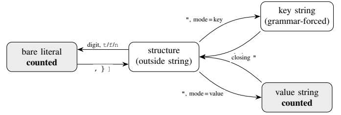
Fig. 1. The JsonPos tracker. Only tokens that land in the two shaded states contribute surprisal; keys and punctuation, which the grammar forces, are ignored. Within the structure state, { pushes an object and sets mode=key , [ pushes an array and sets mode=value , : sets mode=value , , sets mode=key inside an object and value inside an array, and ] ] pop. Backslash escapes inside strings are consumed without leaving the string state.
