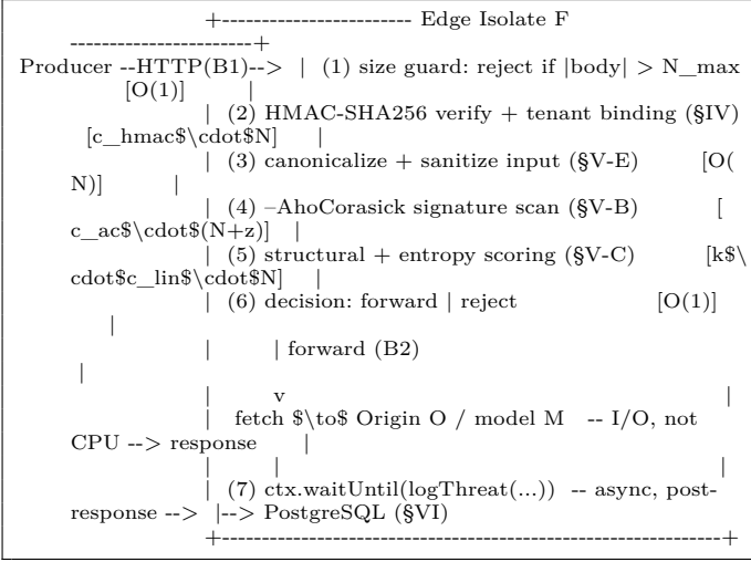
Fig. 1. Request lifecycle in the edge isolate. Steps (1)–(6) are the CPU-bounded critical path analyzed in §III-C; the origin fetch and the waitUntil-deferred threat log (§VI) are I/O and do not accrue against the CPU limit. Steps (2), (4), (5) are the substance of §IV and §V; the size guard (1) supplies the N_{\max} bound that makes the latency analysis absolute.
