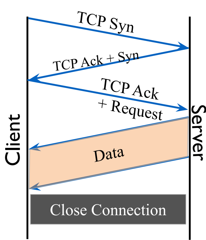
Non-Persistent Connection
