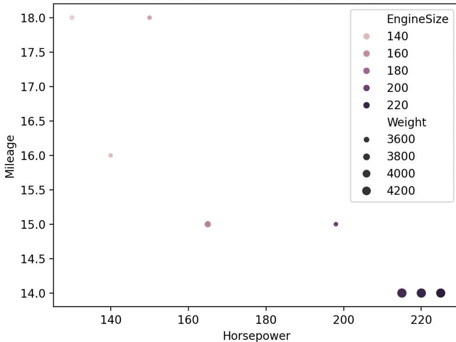
Multivariate Scatter Plot of Car Dataset
