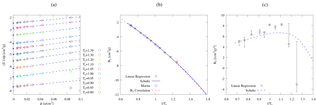
Figure 8: Panel a ) shows the plot of (Z - 1)/\rho with respect to \rho for TraPPE-UA ethane. Blue solid squares represent Schultz’s B_2 values. [45]. Blue dashed lines represent Schultz values of B_2 (intercept) and B_3 (slope). Circles and diamonds are NVT state points simulated with the GOMC package [35]. Using circles in a ) suffices to obtain accurate virial coefficients, therefore diamond points are not used in B_2 and B_3 calculations. In panel b ) and c ) black squares represent the median of B_2 and B_3 when circle points \{1,2,3\} , \{1,2,3,4\} , \{2,3,4\} , and \{1,2,4\} from panel a ) were used in linear regression according to Eq.(27). Error bars represent bootstrapped uncertainties. The blue circles in panel b ) represent B_2 values obtained by Martin and Siepmann [4] using a Monte Carlo method [48].
