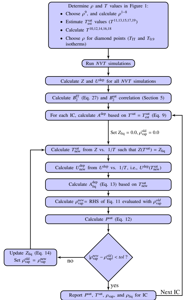
Figure 2: Algorithm to obtain VLE from NVT simulations using ITIC method
