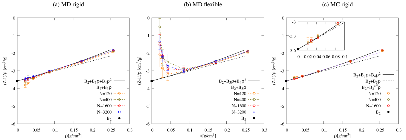
Figure 9: Effect of number of ethane molecules on compressibility factor at low densities at T^{\text{IT}} = 360 . Panel a ) is from MD with rigid bonds (using SHAKE algorithm in LAMMPS), panel b ) is from MD with flexible bonds (harmonic potential using multiple-time-step algorithm RESPA [52] algorithm), and panel c ) is from MC with rigid bonds (GOMC). Solid black lines represent B_2 + B_3\rho + B_4\rho^2 curve where B_{2-4} are obtained from Schultz's work [45]. Dashed black lines represent B_2 + B_3\rho line where B_{2-3} are obtained from Schultz's work. Solid black circle shows the Schultz's value of B_2 . Dashed purple lines represent B_2 + B_3^{\text{eff}}\rho where B_2 and B_3^{\text{eff}} are fit to four lowest density simulation values. Note that the increasing deviation between black line and simulation points at higher densities is due to truncation of virial equation at B_4 . The error bars illustrate the 95 % confidence intervals calculated from four separate runs each consisting two blocks (8 samples). Number of MD steps used to calculate averages is inversely proportional to N with 6 million timesteps for N=120 .
