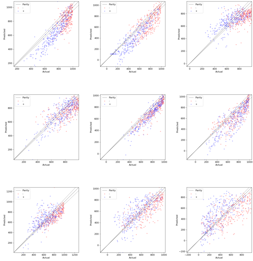
FIG. 1: N_{\text{eff}}
