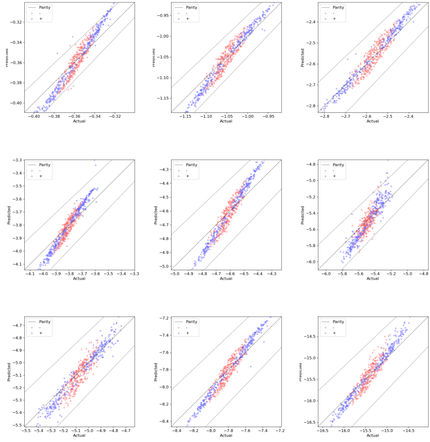
FIG. 2: \hat{U}^{\text{res}}
