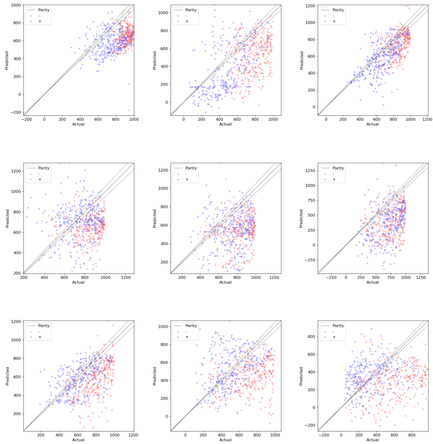
FIG. 1: N_{\text{eff}}
