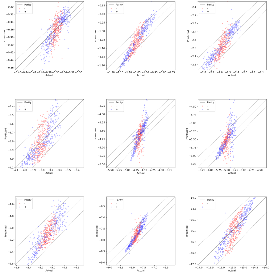
FIG. 2: \hat{U}^{\text{res}}
