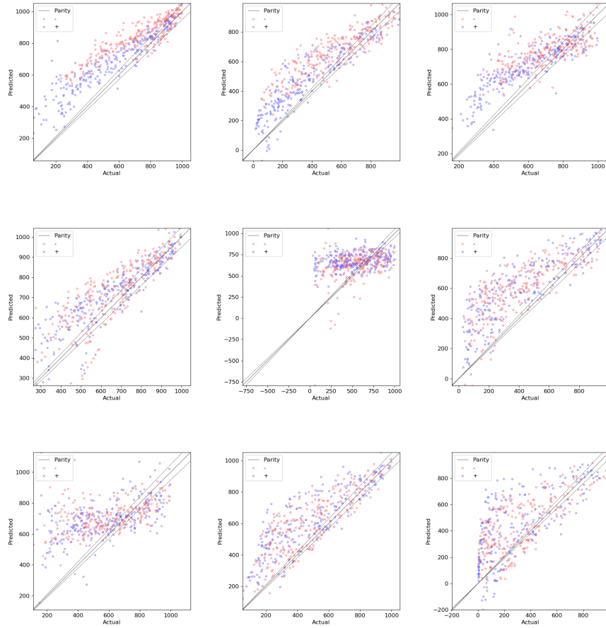
FIG. 1: N_{\text{eff}}
