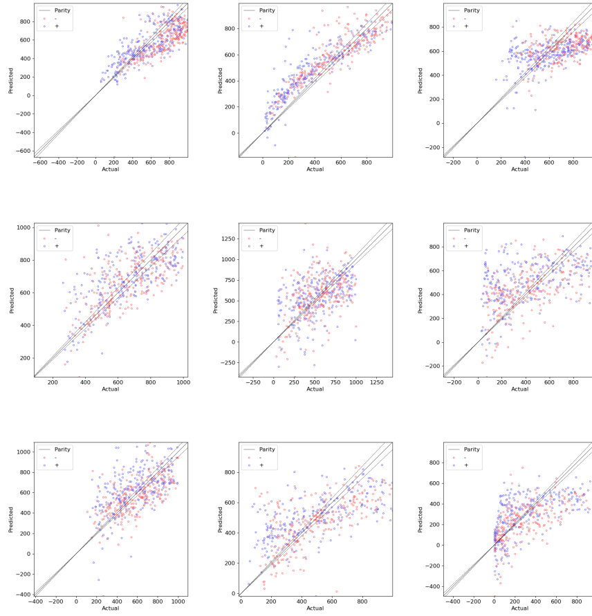
FIG. 1: N_{\text{eff}}
