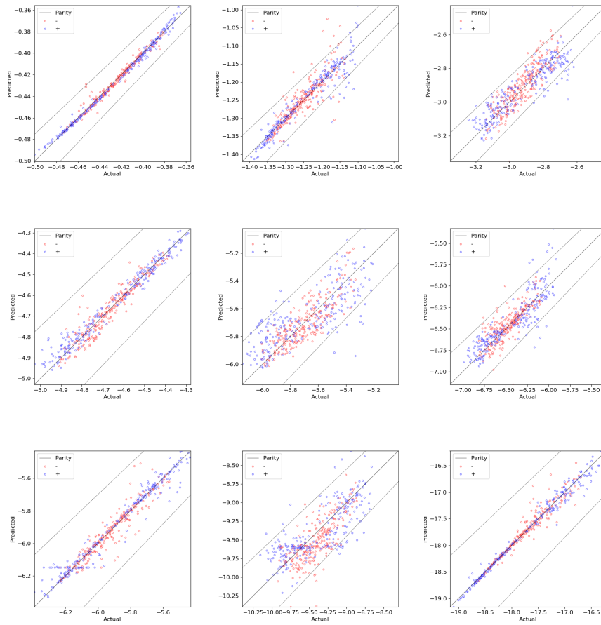
FIG. 2: \hat{U}^{\text{res}}
