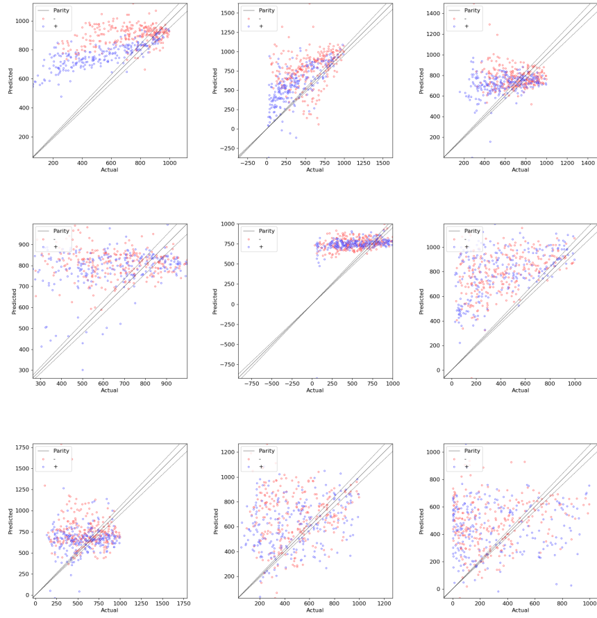
FIG. 1: N_{\text{eff}}
