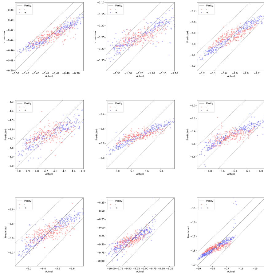
FIG. 2: \hat{U}^{\text{res}}
