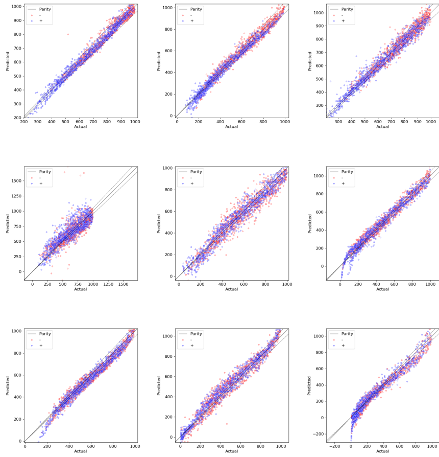
FIG. 1: N_{\text{eff}}
