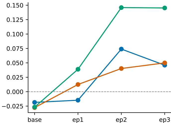
key-fact recall
