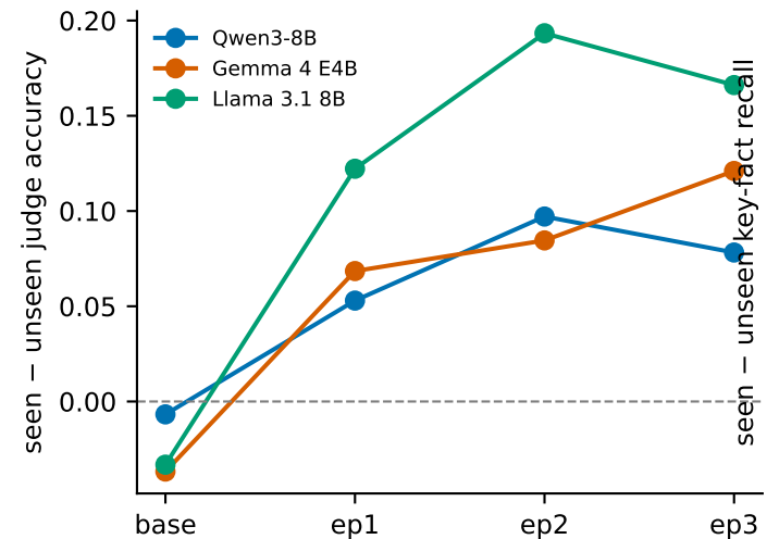
judge accuracy
