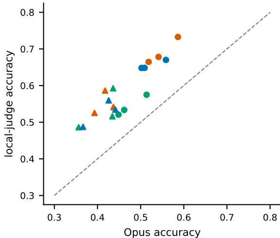
system level: r = 0.90
