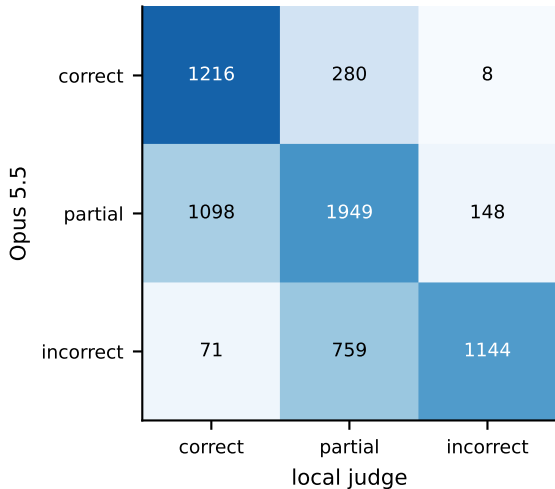
TEST items, \kappa = 0.45
