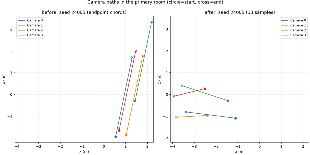
Figure 3: Seed 24005 before and after the group/path diversity constraints. Starts are circles, endpoints crosses.
