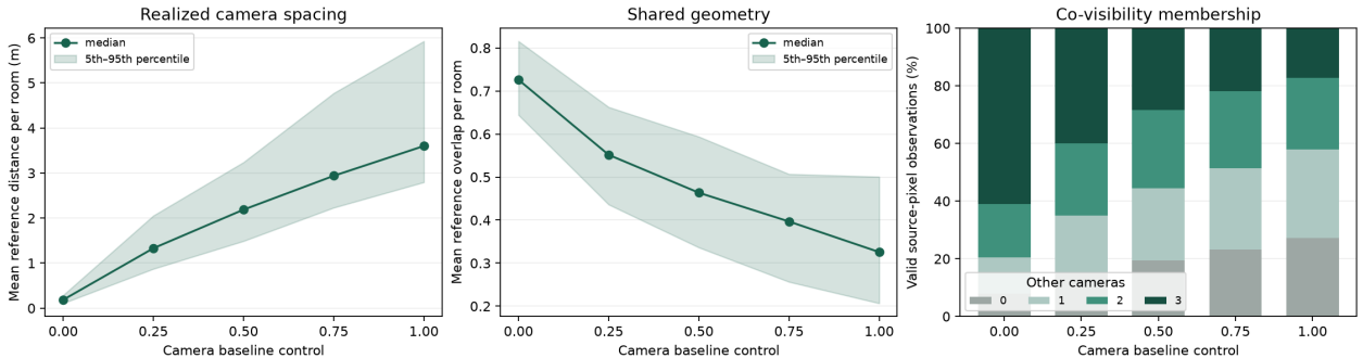
Figure 10: Realized spacing, room-level overlap quantiles and co-visibility cardinality versus the camera-baseline parameter. Pixel observations and views from the same room are correlated.
