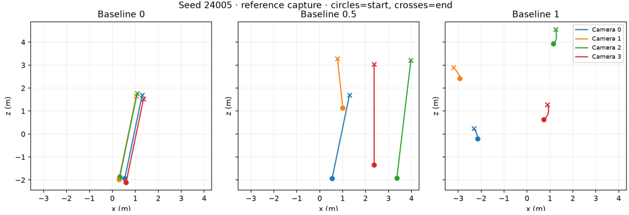
Figure 11: Camera programs for one fixed reference room at three baseline settings, using common metric axes.
