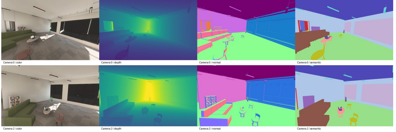
Figure 16: Selected reference room, seed 24005: RGB, metric-depth visualization, view-space normals and semantic labels for cameras 0 and 2 at the same time. Camera selection and pixel-aligned annotation comparisons are interactive on the project page. These illustrations are separate from the consecutive population evaluation.
