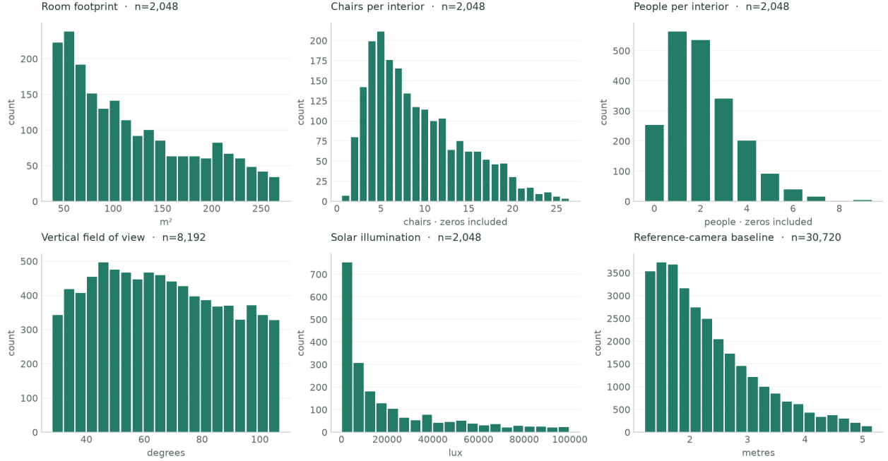
Figure 14: Absolute distributions in the camera-baseline reference population of 2,048 rooms at the default camera baseline. Each panel preserves its denominator and units.
