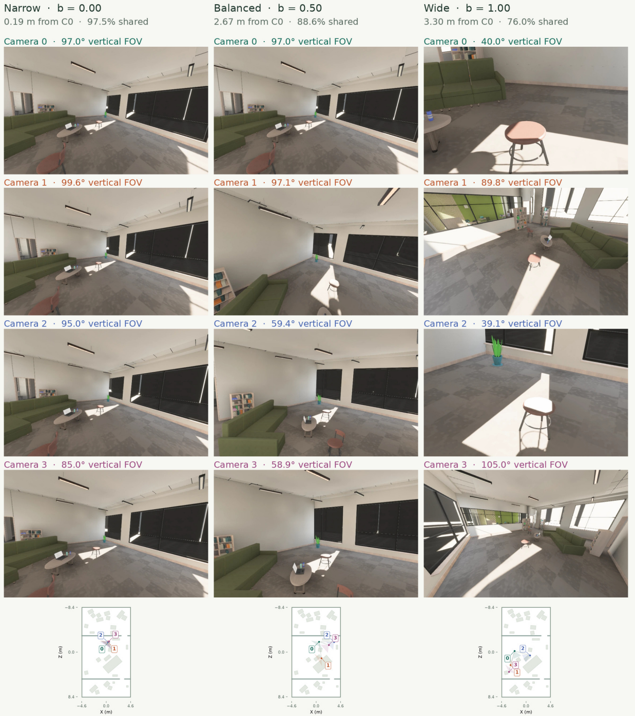
Figure 12: Fixed sunlit seating scene (seed 24005), with narrow, balanced and wide baseline policies from left to right. Rows retain cameras 0–3 in order; the bottom row locates their centers in the same primary room. Close views concentrate on similar content; wider sampling changes perspective and the surfaces jointly observed. Header values describe these particular captures, not population averages.
