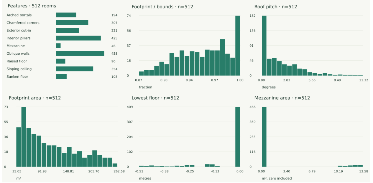
Figure 7: Architectural feature counts and continuous parameter distributions from the complete population; absent features are retained.
