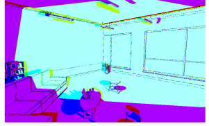
Mask · 98.9% shared
