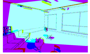
Mask · 98.9% shared
