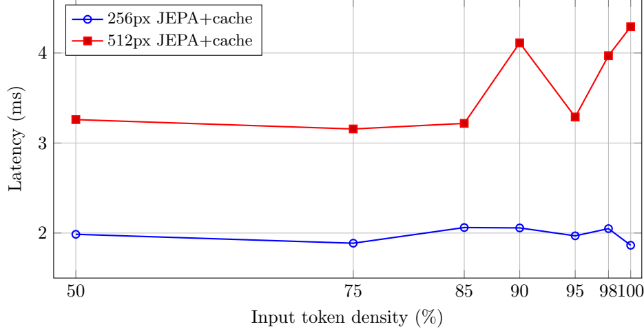
Figure 1: WGPU sparsity-latency sweep for the Bevy-style tiny JEPA+feature-cache path. The 100% point is the dense ordered baseline.
