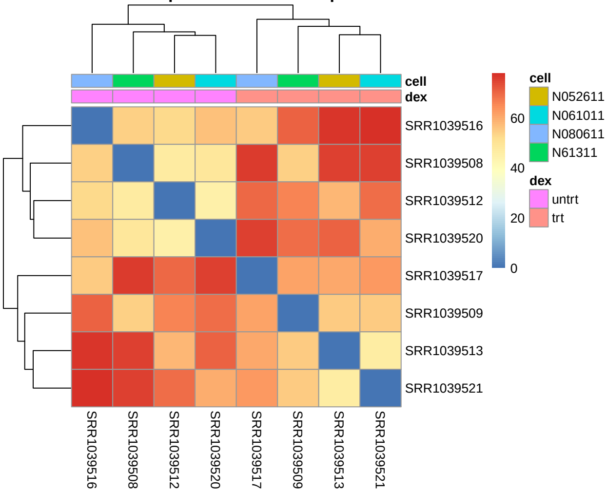
Sample distance heatmap
