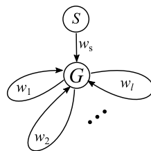
図 XII.4.7 G(V, E)
