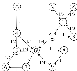
図 XIII.4.1 G(V, E)
