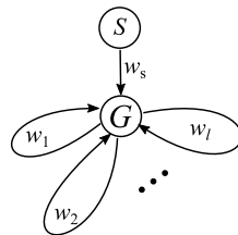
図 XII.4.7 G(V, E)
