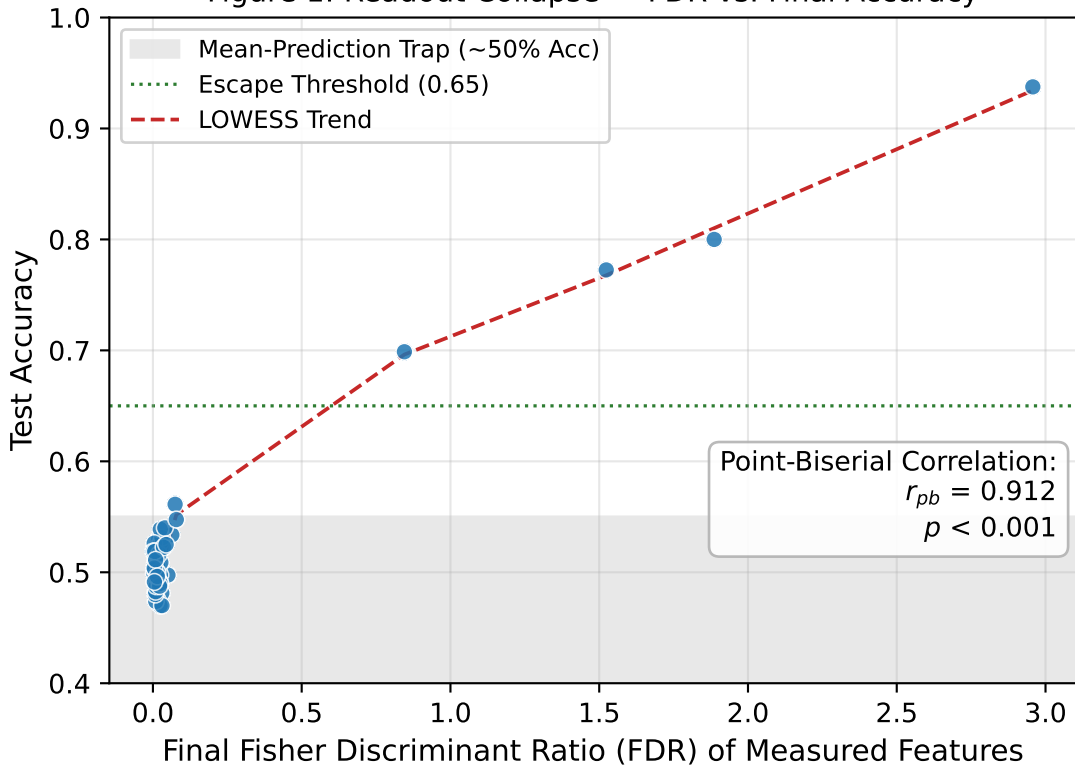
Figure 1: Readout Collapse — FDR vs. Final Accuracy
