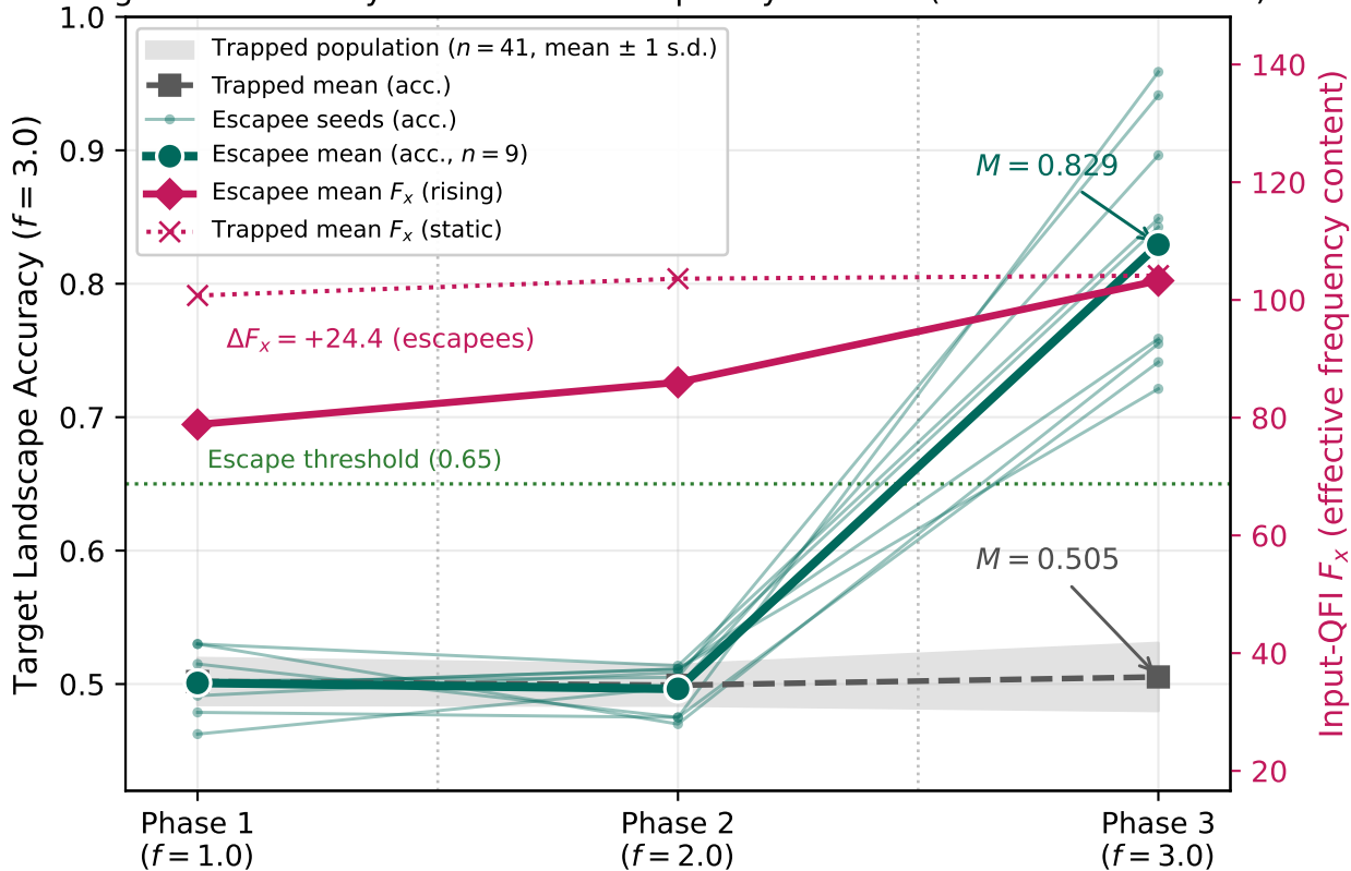
Figure 4: Accuracy and Effective Frequency Content (Forward Curriculum)
