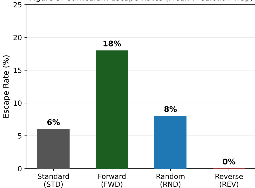
Figure 3: Curriculum Escape Rates (Mean-Prediction Trap)
