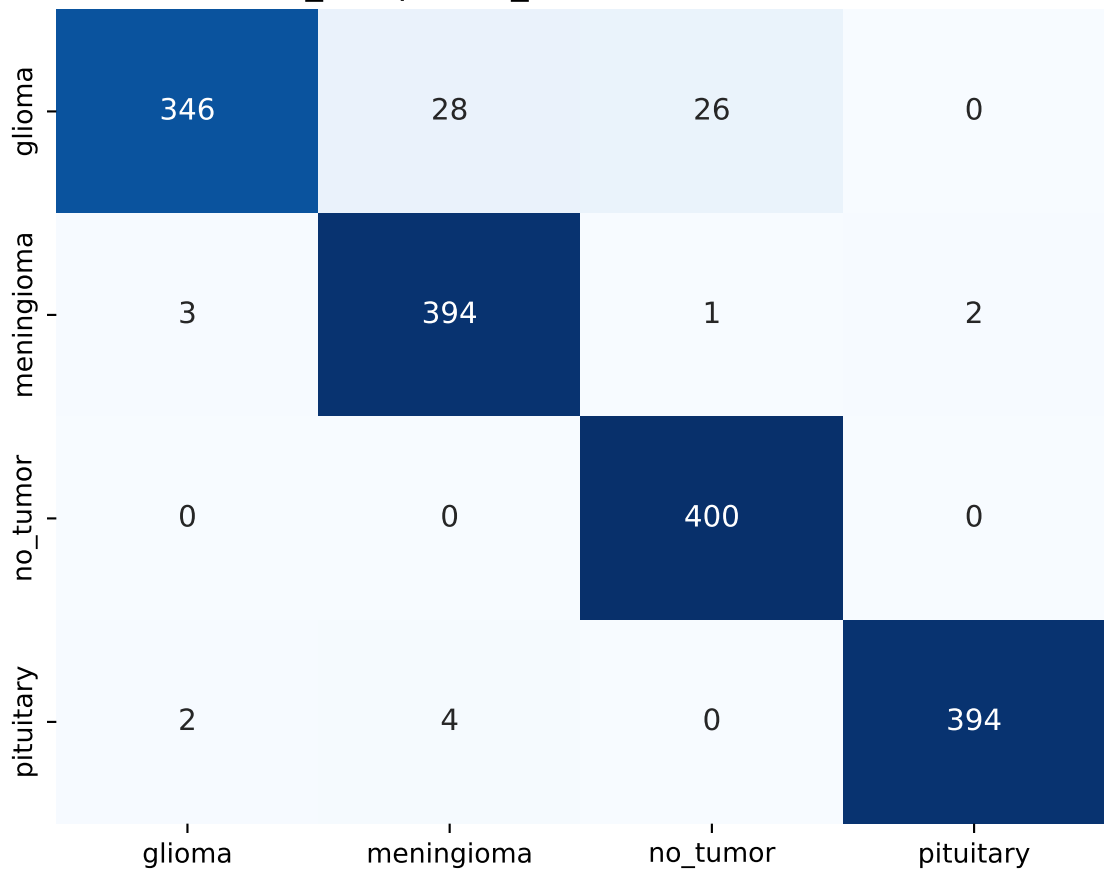
ResNet50_Nickparvar_baseline — Confusion Matrix
