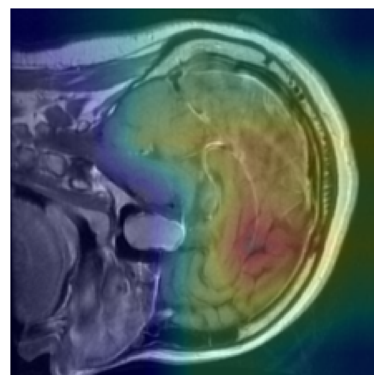
Pred: Pituitary (100.0%)
