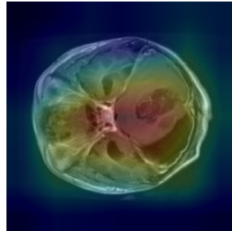
Pred: Glioma (100.0%)
