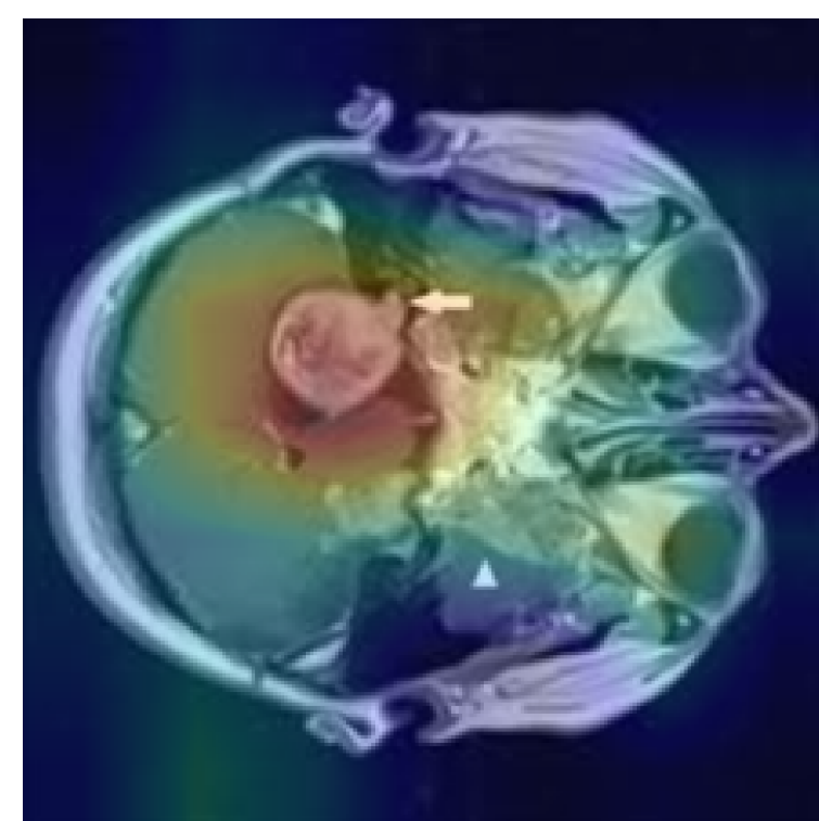
Pred: Meningioma (60.6%)
