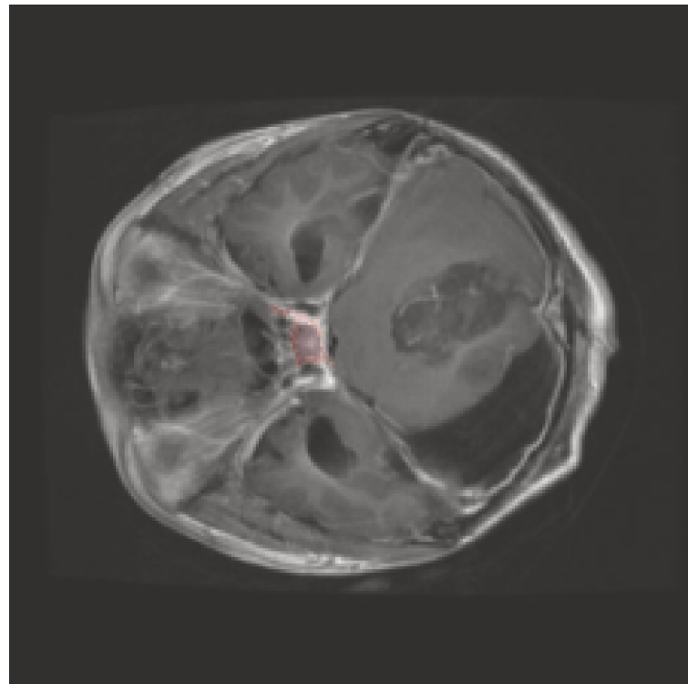
Expert Mask
