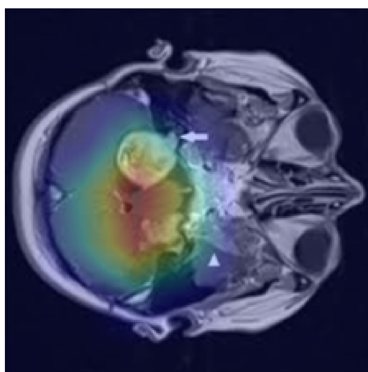
Pred: Meningioma (98.8%)
