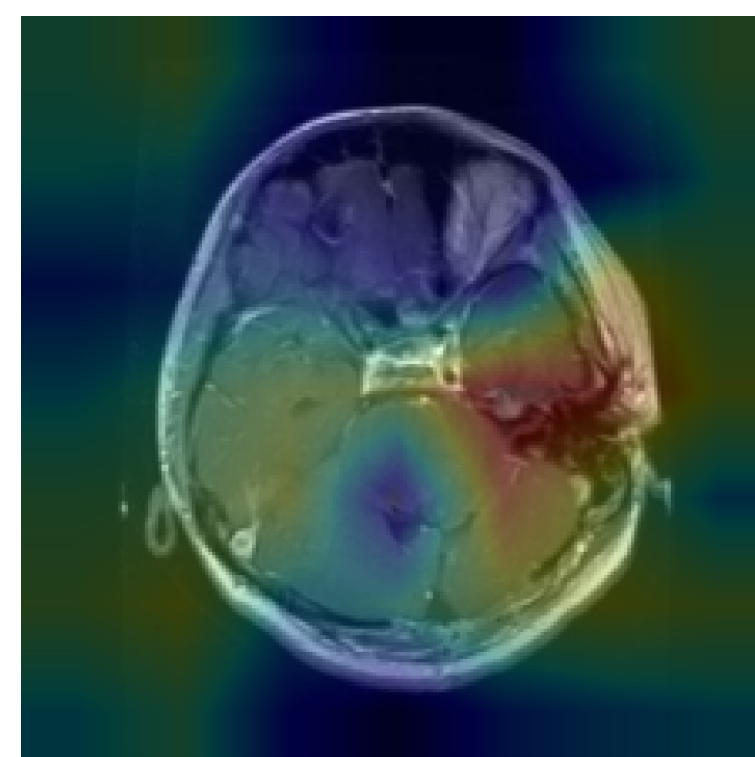
Pred: Glioma (100.0%)
