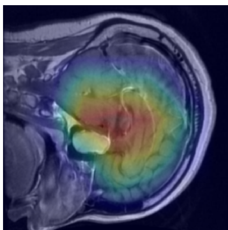
Pred: Pituitary (100.0%)
