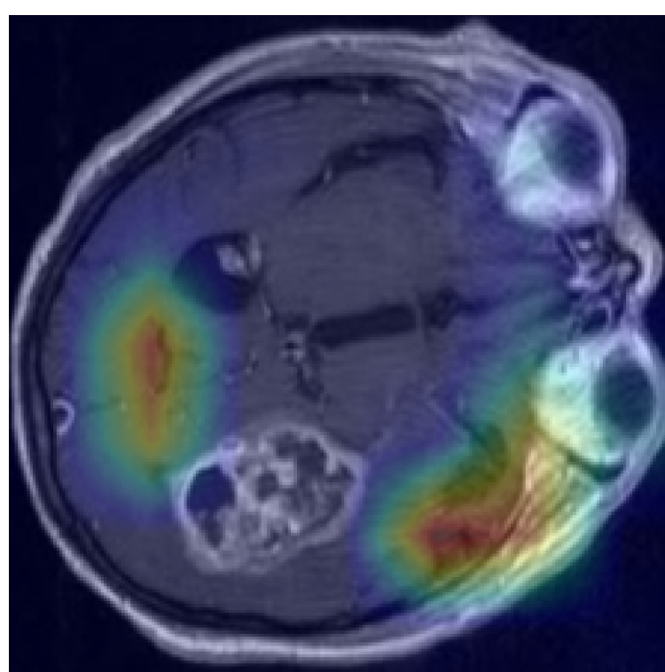
Pred: Meningioma (73.8%)
