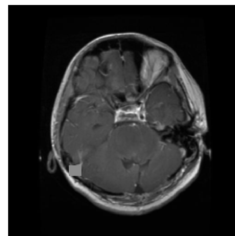
Pred: Glioma (100.0%)
