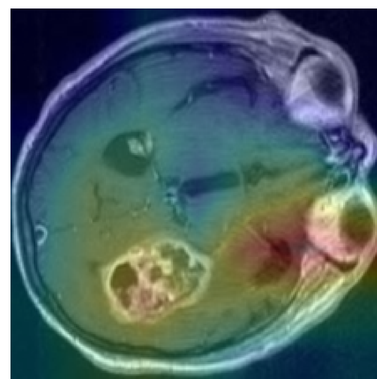
Pred: Meningioma (99.5%)
