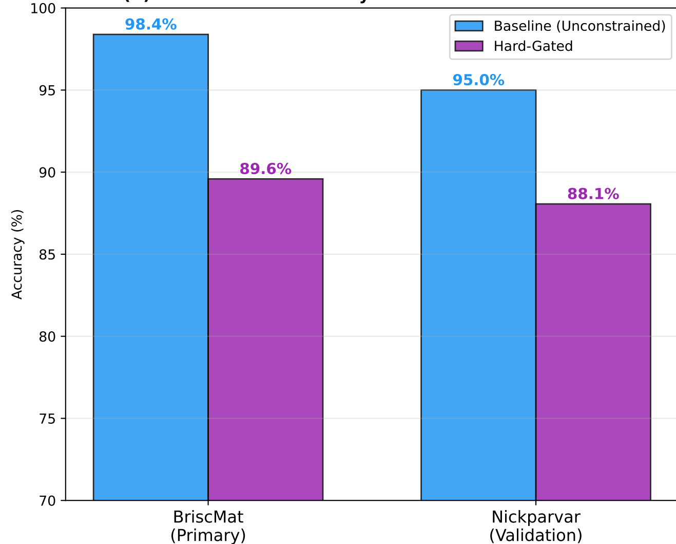
(B) Classification Accuracy — Baseline vs. Hard-Gated
