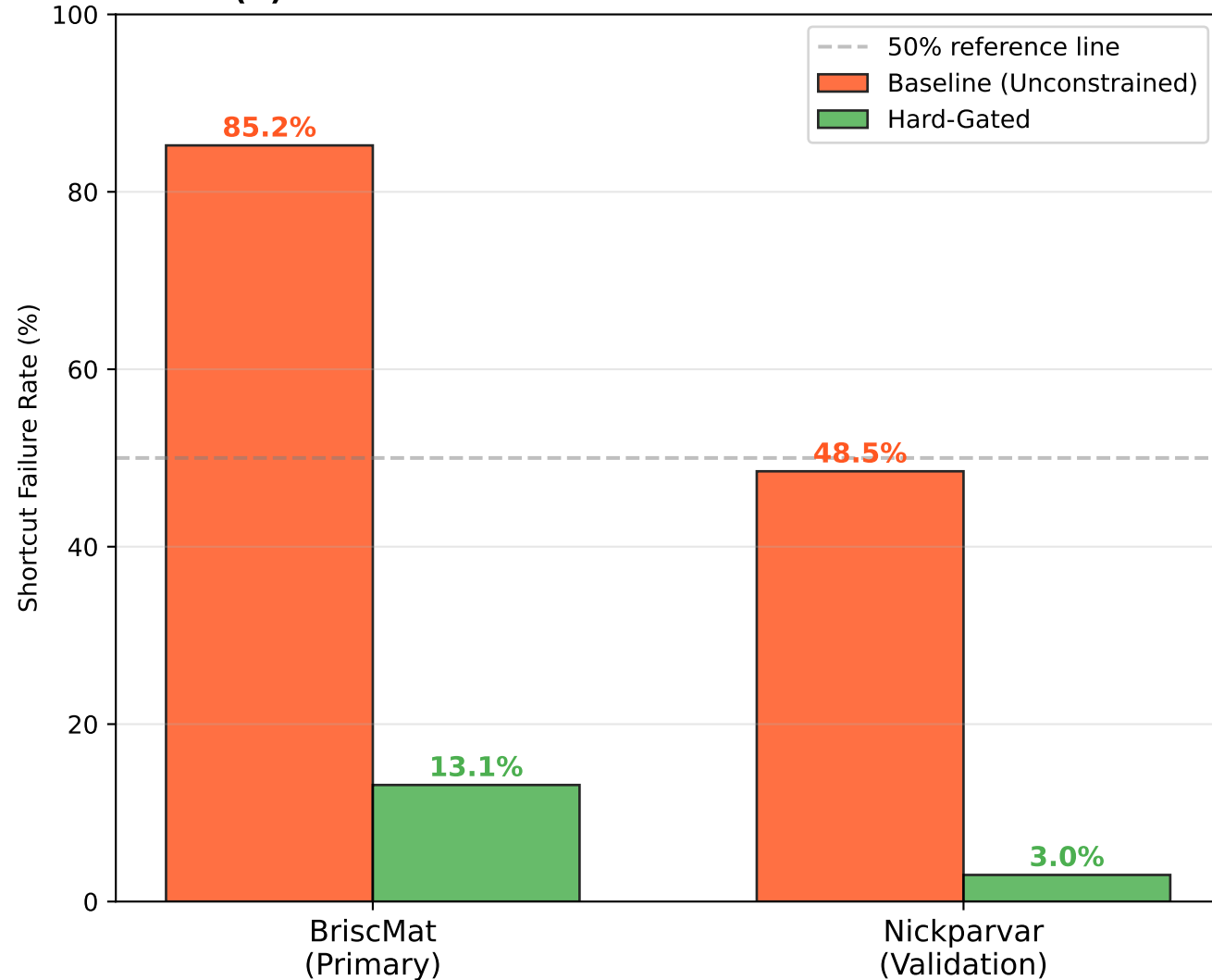
(A) Shortcut Failure Rate — Baseline vs. Hard-Gated
