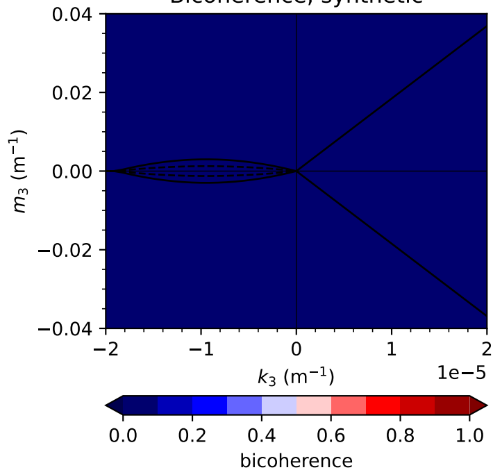
Bicoherence, synthetic
