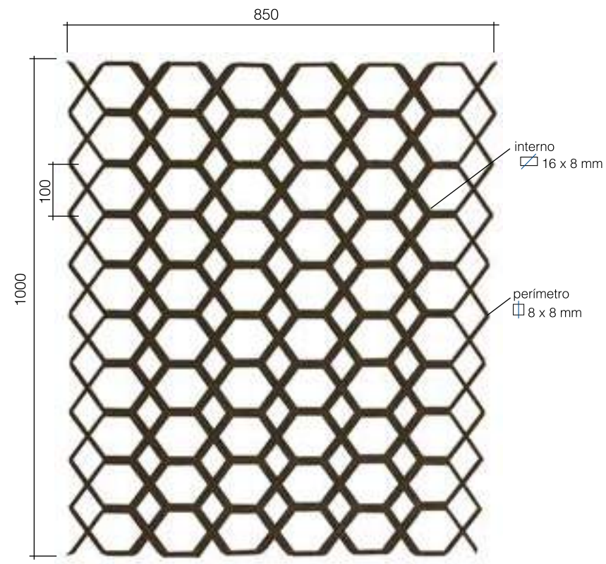
Art. GD299/1 8 x 8 mm + 16 x 8 mm L 850 mm H 1000 mm
