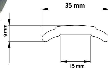
Art. 810/B/1T L 3000 mm
