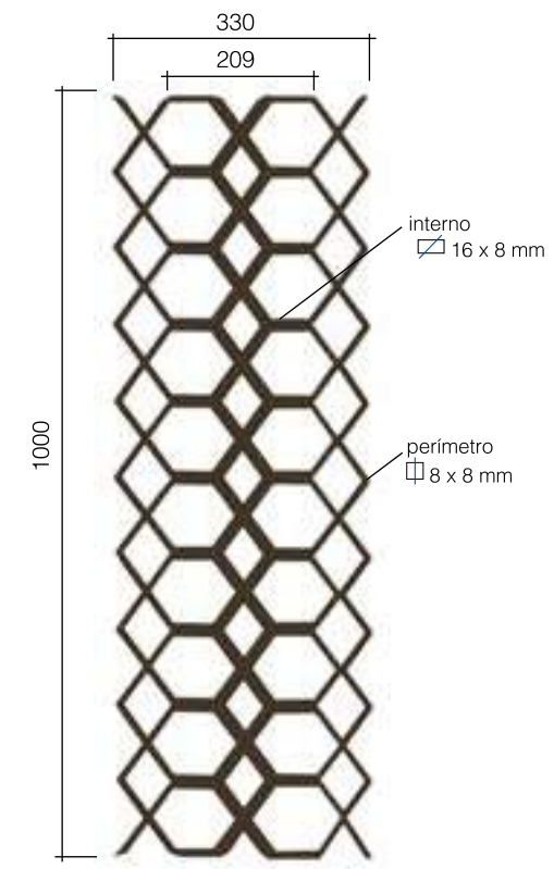
Art. GD299/2 8 x 8 mm + 16 x 8 mm L 330 mm H 1000 mm
