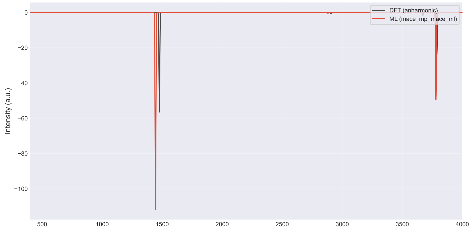
IR Spectrum Comparison: mace_mp_mace_ml vs DFT
