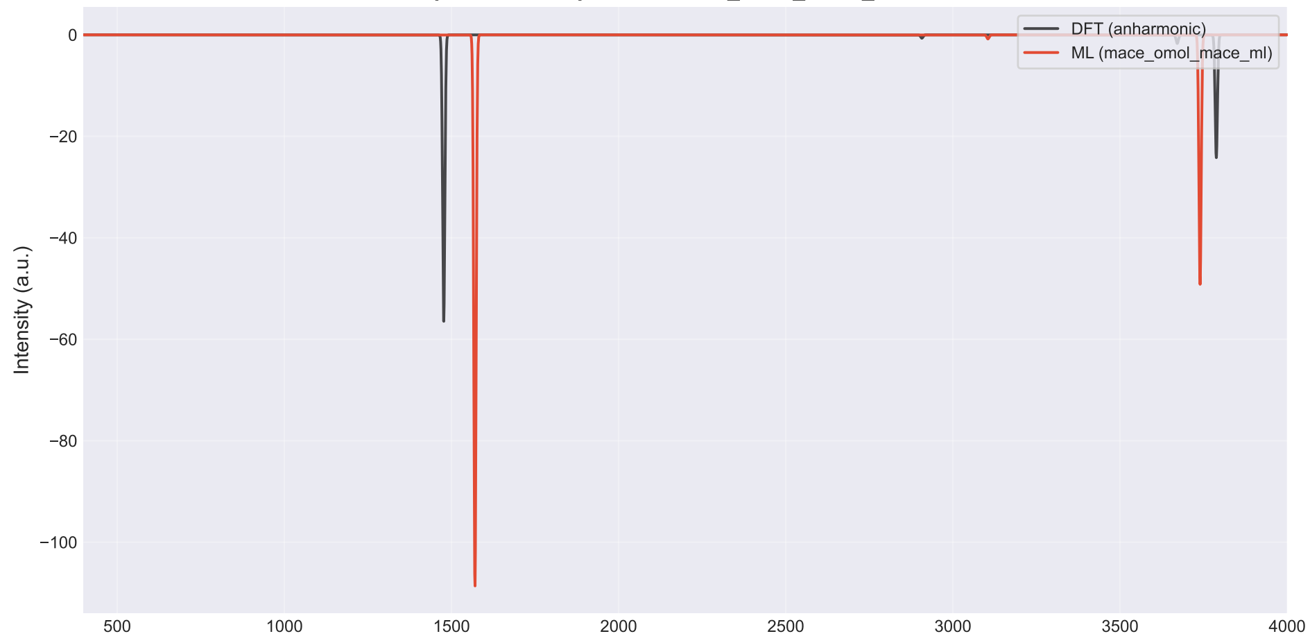
IR Spectrum Comparison: mace_omol_mace_ml vs DFT
