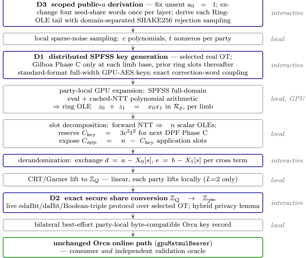
Figure 2: The live forward-FC pipeline; both parties run it as independent processes on distinct GPUs. Blue-framed stages exchange messages over TCP; all other stages are party-local, and Ring-LPN expansion runs on the GPU. The unchanged online consumer runs only in the post-exit checker for this artifact. The transport is loopback and unauthenticated.
