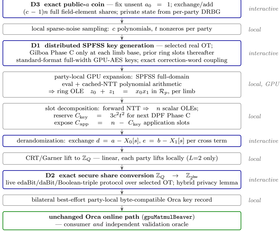
Figure 2: The live forward-FC pipeline; both parties run it as independent processes on distinct GPUs. Blue-framed stages exchange messages over TCP; all other stages are party-local, and Ring-LPN expansion runs on the GPU. The unchanged online consumer runs only in the post-exit checker for this artifact. The transport is loopback and unauthenticated.
