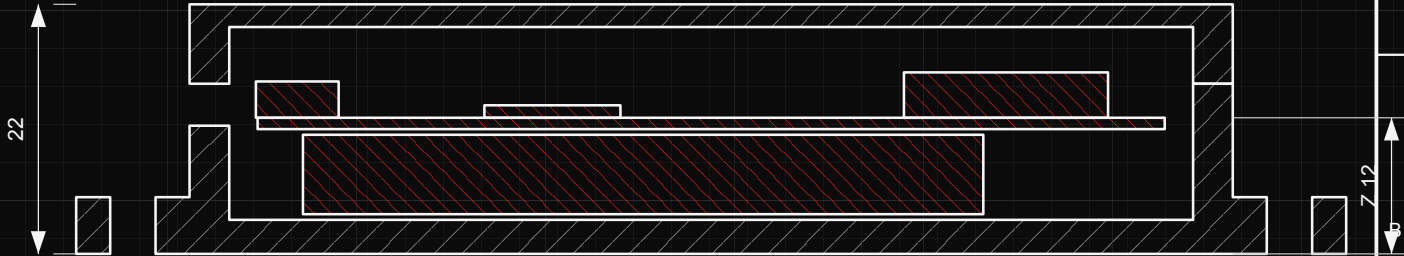
SECTION A-A / Y = +8 / 1.5:1 Enclosure white hatch, electronics red hatch (PCB1, U1, U7, J1, BT1)
