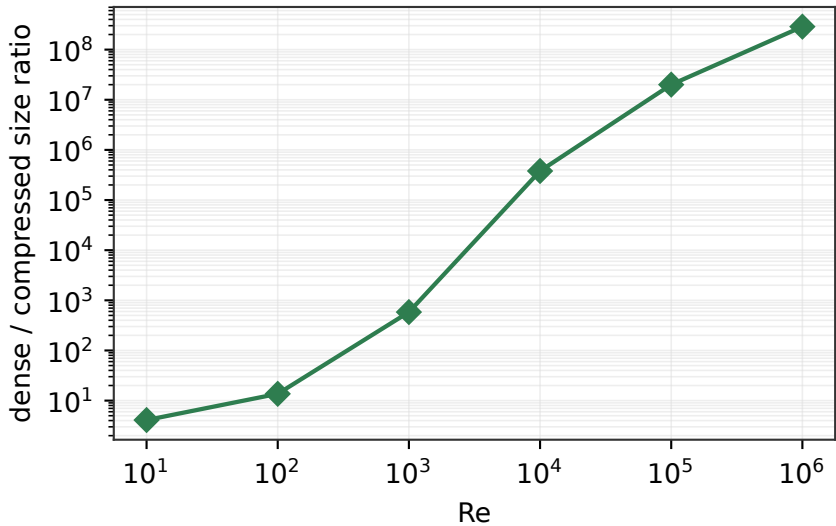
QTT compression ratio, full pre-registered Re grid
