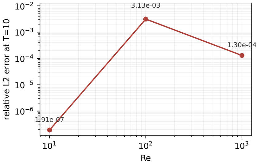
Error scaling vs Re (post temporal-order fix)
