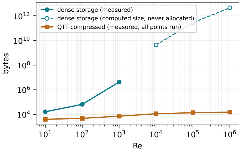
Memory / qubit count vs Re
