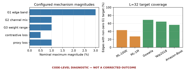
Fig. 2. Python-generated code-level diagnostics. Left: configured nominal magnitudes (not commensurate causal effects). Right: one-refresh target coverage at L=32 ; orange MovieLens bars are upper bounds and green sparse-data bars are exact. This figure contains no corrected model outcome.
