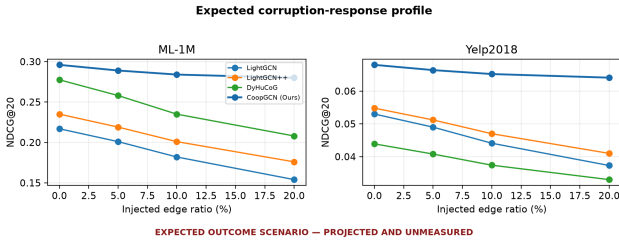
Fig. 4. Expected corruption-response scenario generated from data/expected\oise.csv. Values are projected and unmeasured.
