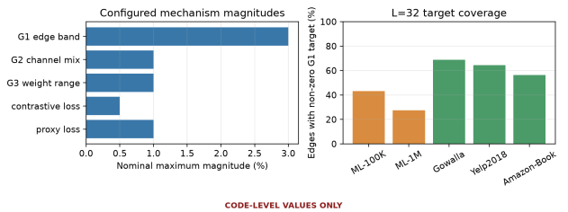
Fig. 5. Python-generated code-level diagnostics. Left: configured nominal magnitudes (not commensurate causal effects). Right: one-refresh target coverage at L=32 ; orange MovieLens bars are upper bounds and green sparse-data bars are exact. This figure reports code-level values only.
