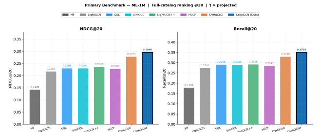
Fig. 2. Primary benchmark on ML-1M: \text{NDCG@20} (left) and \text{Recall@20} (right) for all eight models under full-catalogue ranking at cut-off 20. † denotes projected values.
