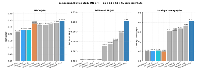
Fig. 5. Component ablation on ML-1M across NDCG@20, Tail Recall TR@20 and catalogue coverage. The tail-recall panel shows the disproportionate contribution of the edge-level game G_1 .
