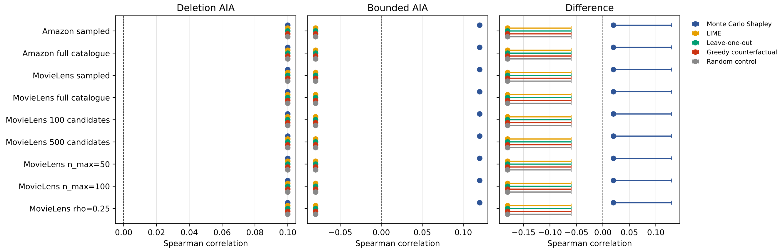
AIA components and Actionability Gap (singleton estimand; budgets excluded)
