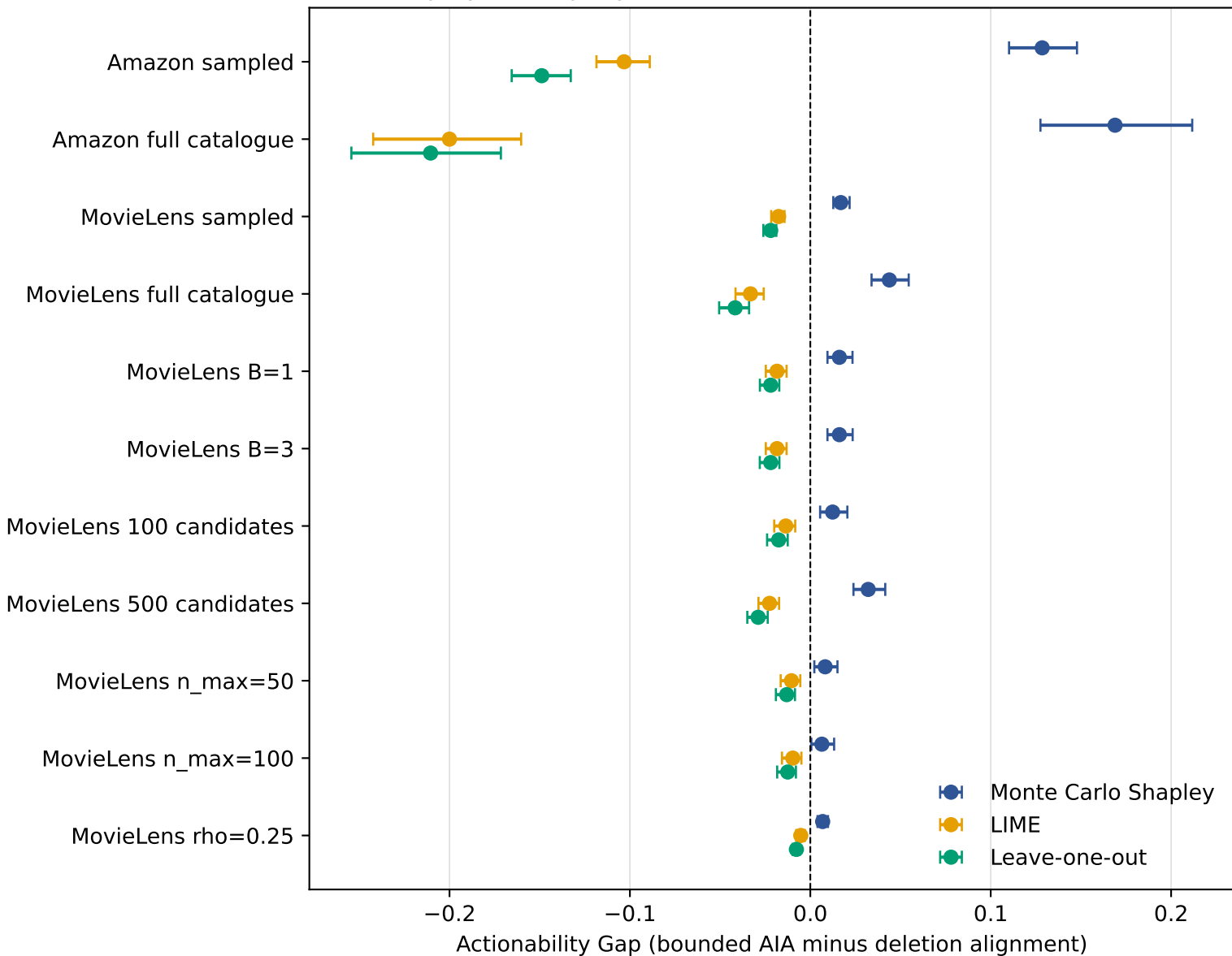
Shapley is uniquely intervention-robust across 11 conditions
