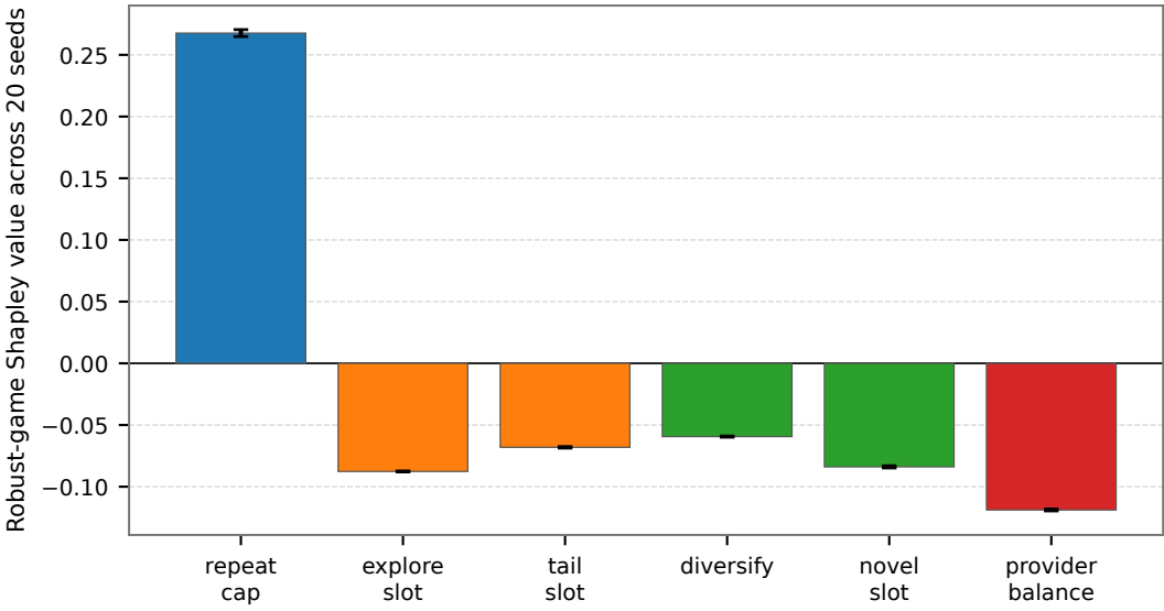
Fig. 2: Exact robust-game intervention attribution
